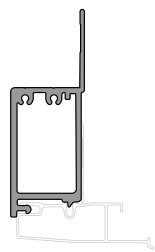
2" FLAT CASING
